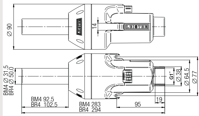
Installation arrangement
